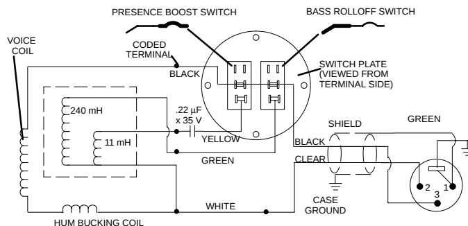
INTERNAL CONNECTIONS
