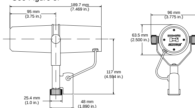
OVERALL DIMENSIONS
